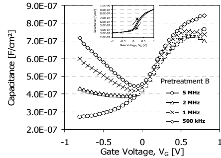
Fig. 12 Room temperature C-V characteristics of Al/ \text{Al}_2\text{O}_3 /AlInSb/InSb MOSCAP with surface pretreatment B
