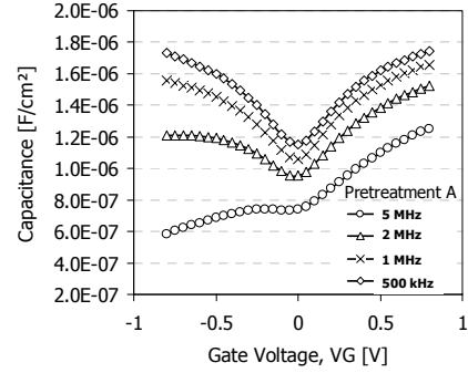
Fig. 11 Room temperature C-V characteristics of Al/ \text{Al}_2\text{O}_3 /AlInSb/InSb MOSCAP with surface pre-treatment A
