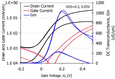
Fig. 10 Transfer characteristics of 85nm L_G e-mode InSb QWFET with L_{SD}=0.75 \mu\text{m} ( V_{DS}=0.5 and 0.05\text{V} )
